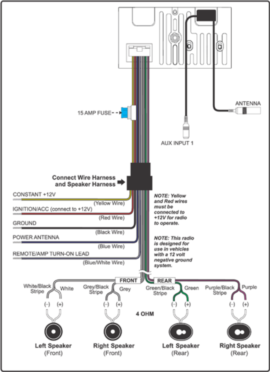
Figure 5 - Wiring Diagram
